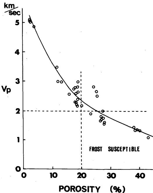
Fig. 2. The relationship between ultra-sonic propagation velocity ( V_p ) and porosity.
