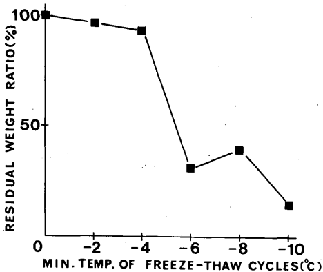
Fig. 5. Dependence of residual weight on freezing temperature.
