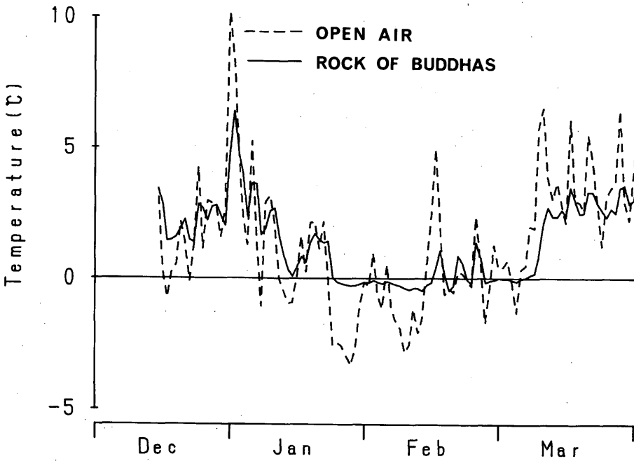
Fig. 12. Temperature fluctuation at Odaka.
