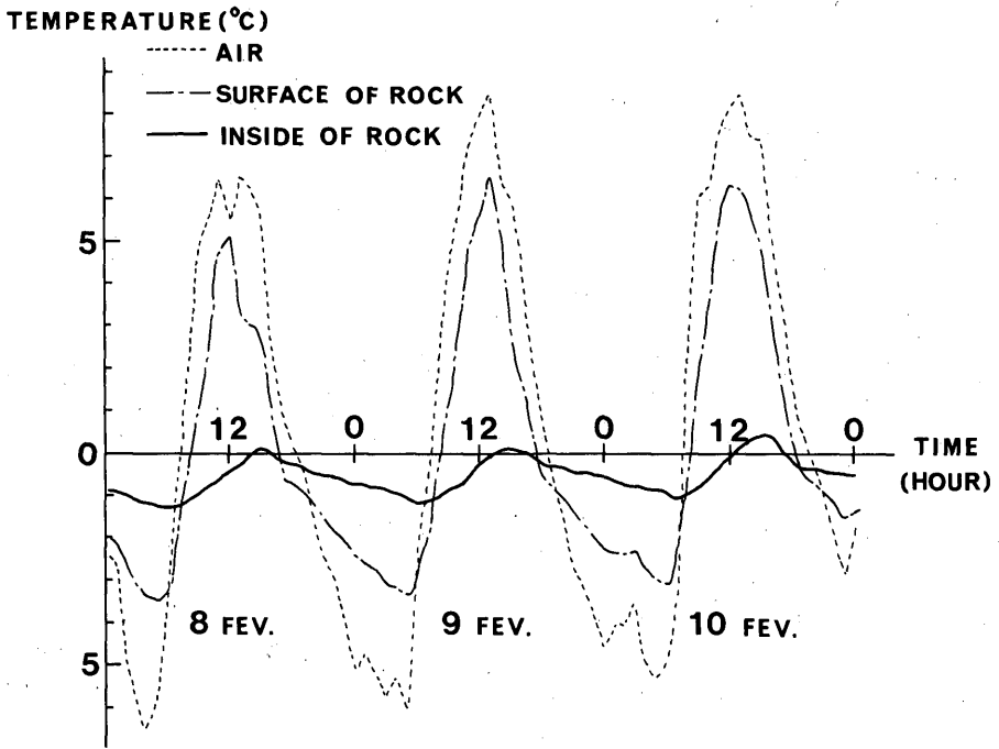
Fig. 8. Temperature changes of a rock specimen in the open-air.
