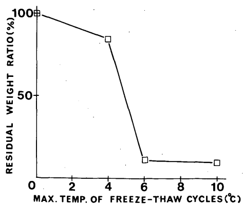
Fig. 6. Dependence of residual weight on thawing temperature.
