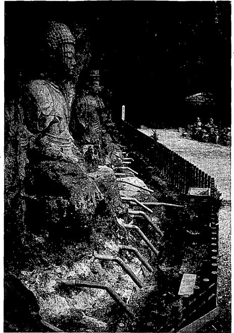
Fig. 4. Pipes and drains for the rock-cliff Buddhas of Usuki, Oita Prefecture.
