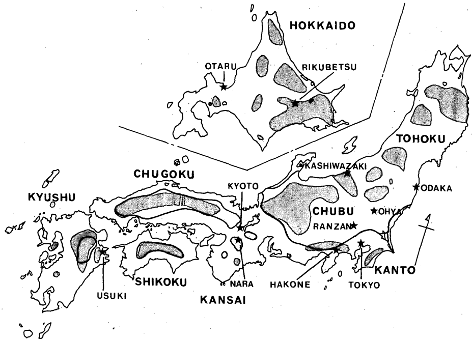
Fig. 10. Distribution of possible areas for frost shattering of stone artifacts. (This is a tentative map based on the AMeDAS data of 1983 Oct.–1984 May. More data might yield a different pattern.)
