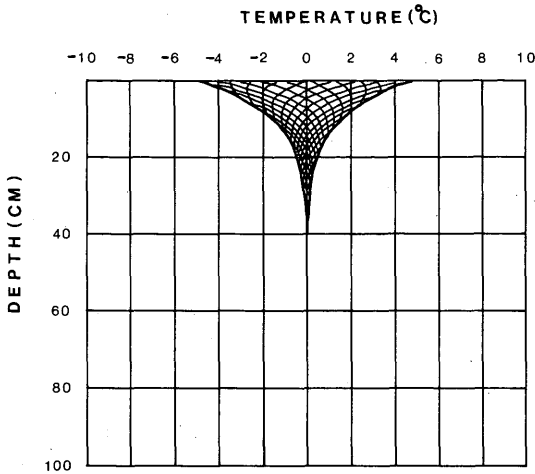
Fig. 7. Temperature fluctuation in bedrock of wet tuff (surface temperature range of +5 to -5°C).
